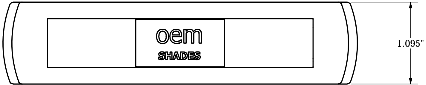
P/N 0219L FRONT VIEW
