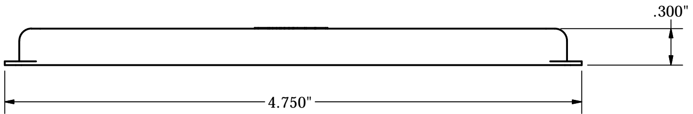
P/N 0219L SIDE VIEW
